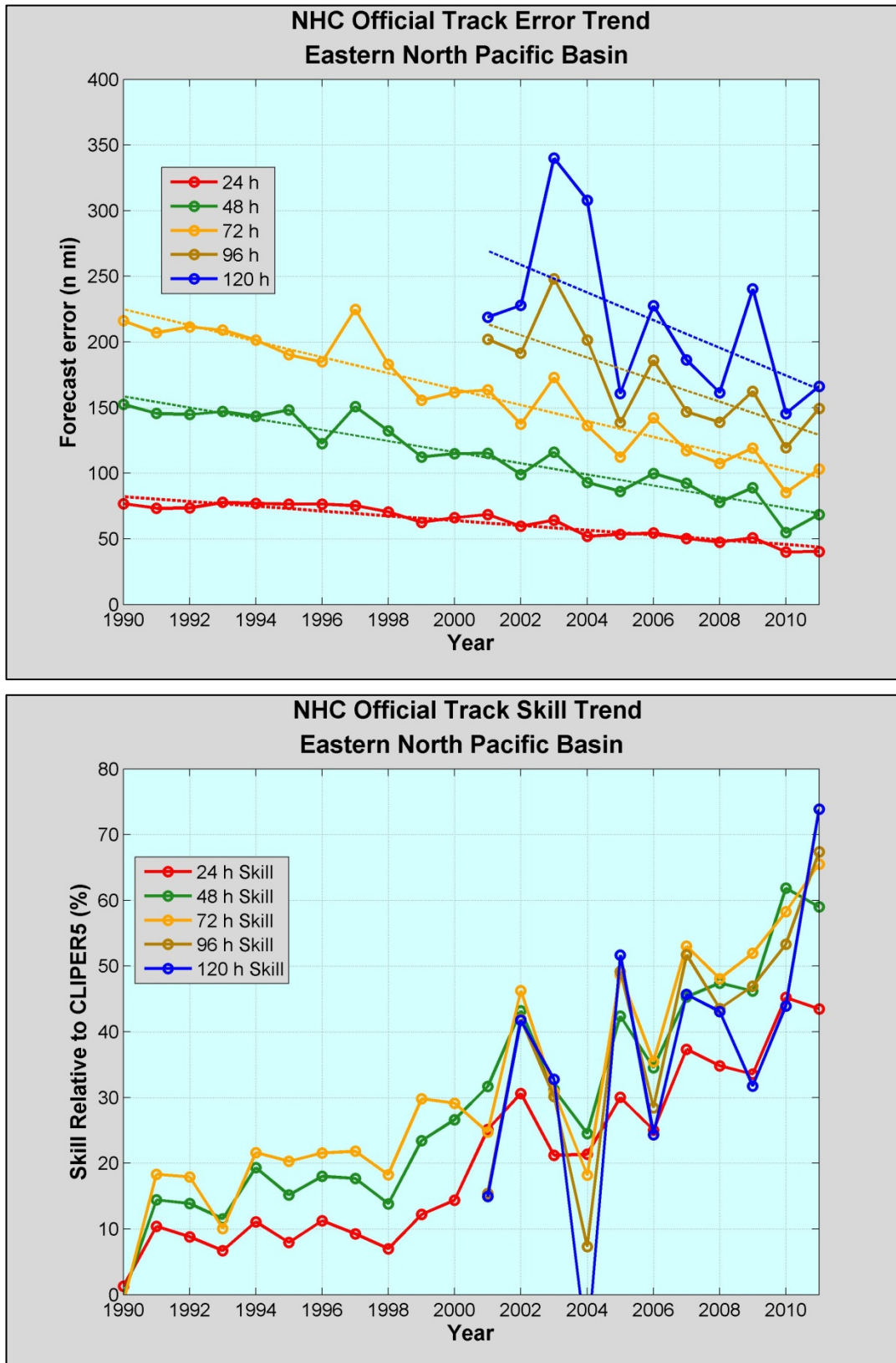
Figure 10. Recent trends in NHC official track forecast error (top) and skill (bottom) for the eastern North Pacific basin.
