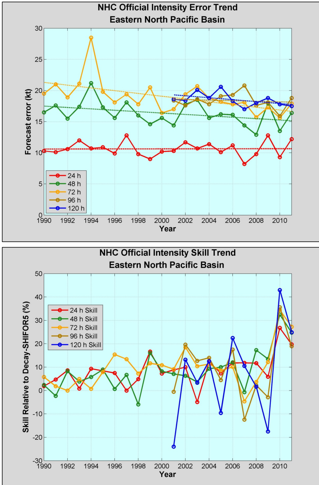
Figure 14. Recent trends in NHC official intensity forecast error (top) and skill (bottom) for the eastern North Pacific basin.
