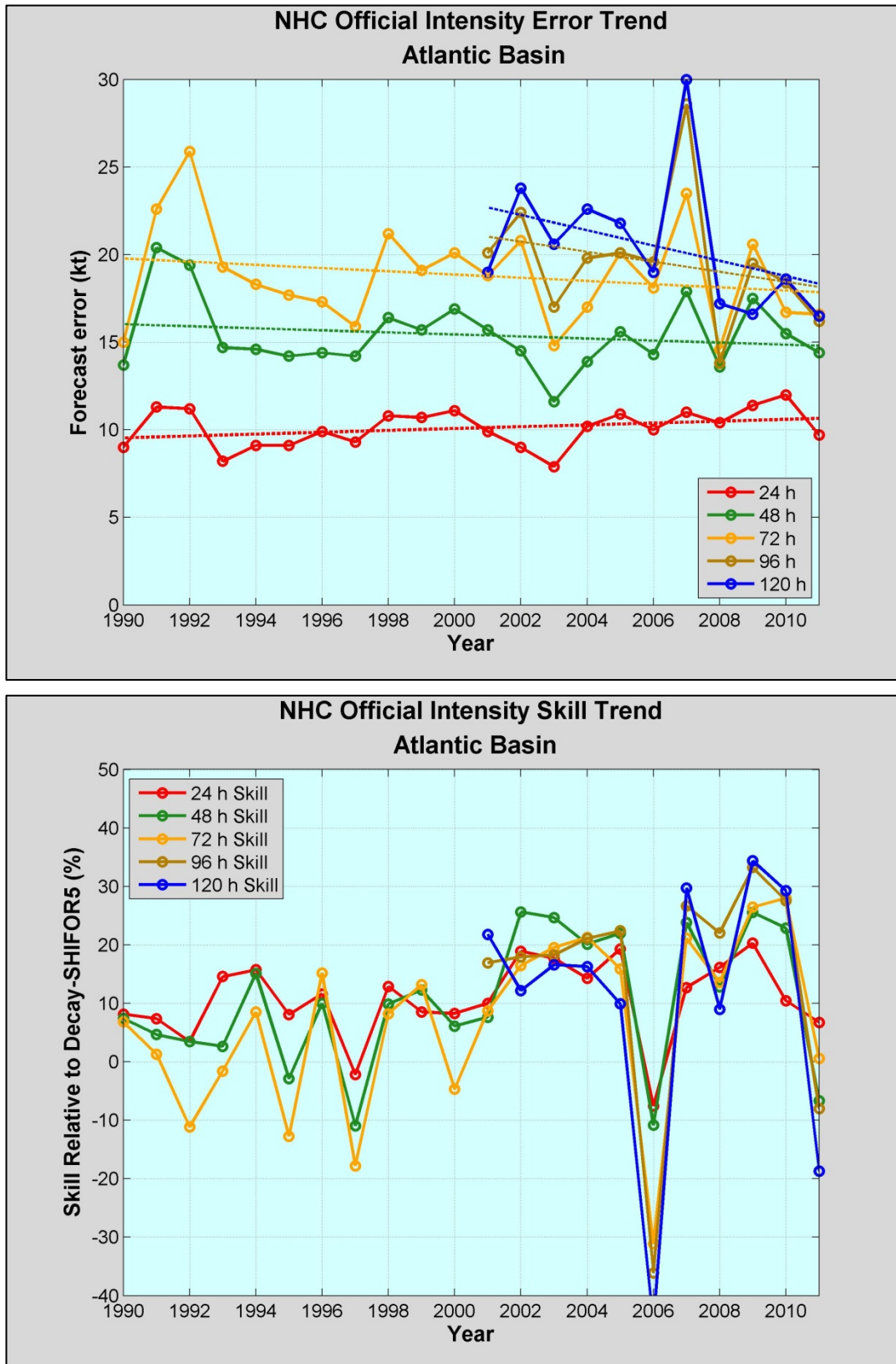
Figure 6. Recent trends in NHC official intensity forecast error (top) and skill (bottom) for the Atlantic basin.
