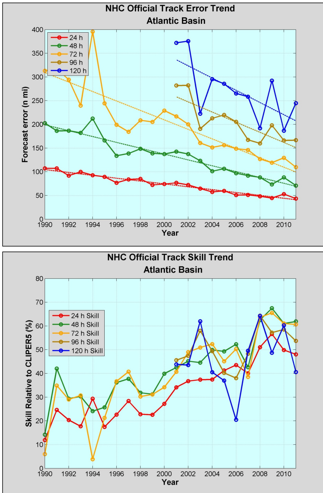
Figure 2. Recent trends in NHC official track forecast error (top) and skill (bottom) for the Atlantic basin.
