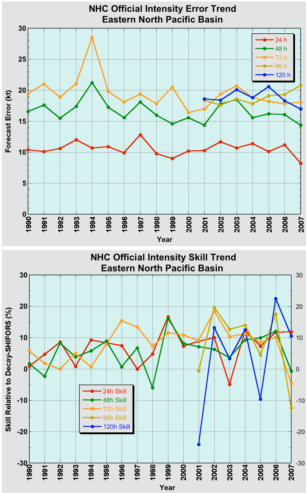
Figure 13. Recent trends in NHC official intensity forecast error (top) and skill (bottom) for the eastern North Pacific basin.
