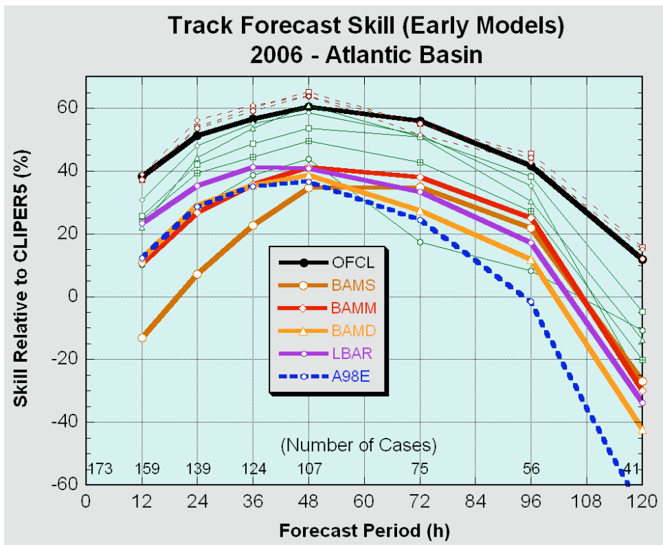
Figure. 2. Homogenous comparison for selected Atlantic basin early track guidance models for 2006. The top panel shows just the more advanced models (which also appear in the bottom panel as thin lines). Simpler models are highlighted in the bottom panel.
