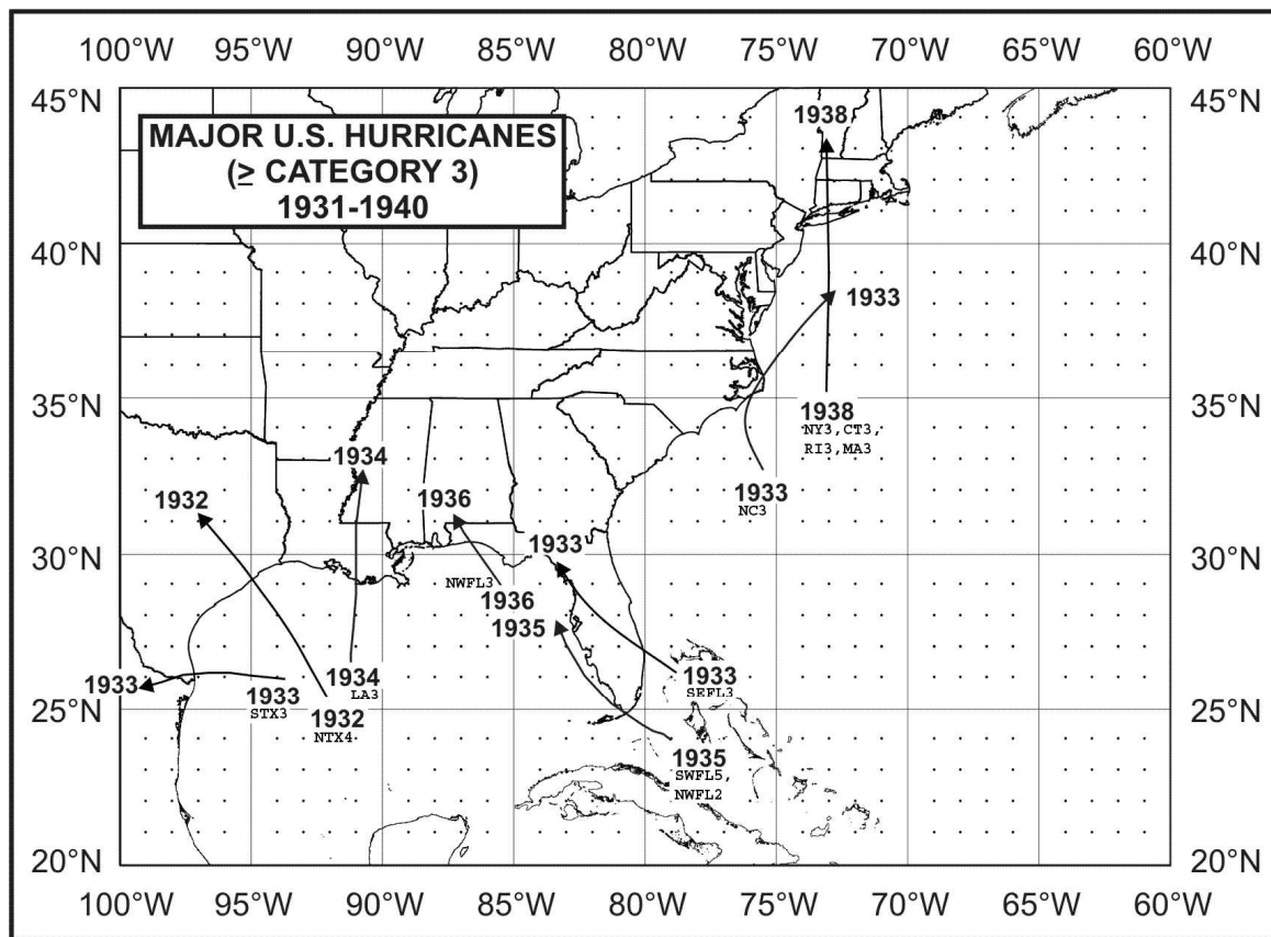
Figure 9. Landfalling United States major hurricanes (stronger than or equal to a category 3) during the period 1931-1940.
