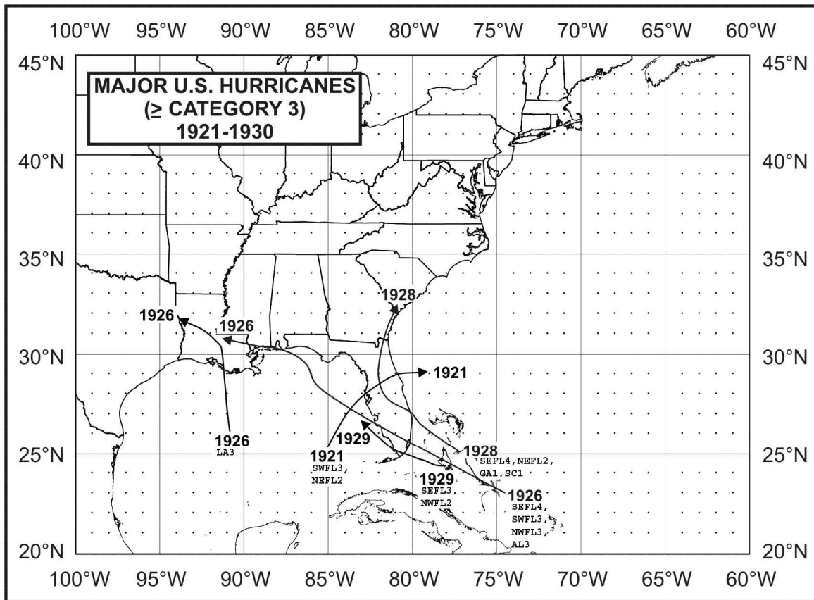
Figure 8. Landfalling United States major hurricanes (stronger than or equal to a category 3) during the period 1921-1930.
