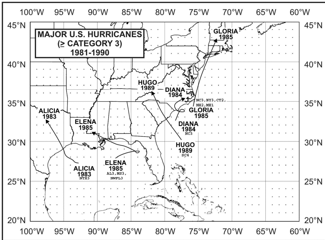
Figure 14. Landfalling United States major hurricanes (stronger than or equal to a category 3) during the period 1981-1990.
