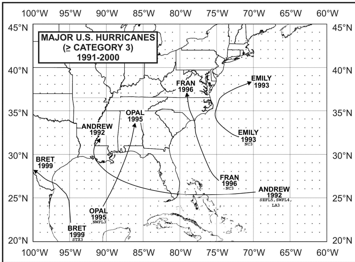
Figure 15. Landfalling United States major hurricanes (stronger than or equal to a category 3) during the period 1991-2000.
