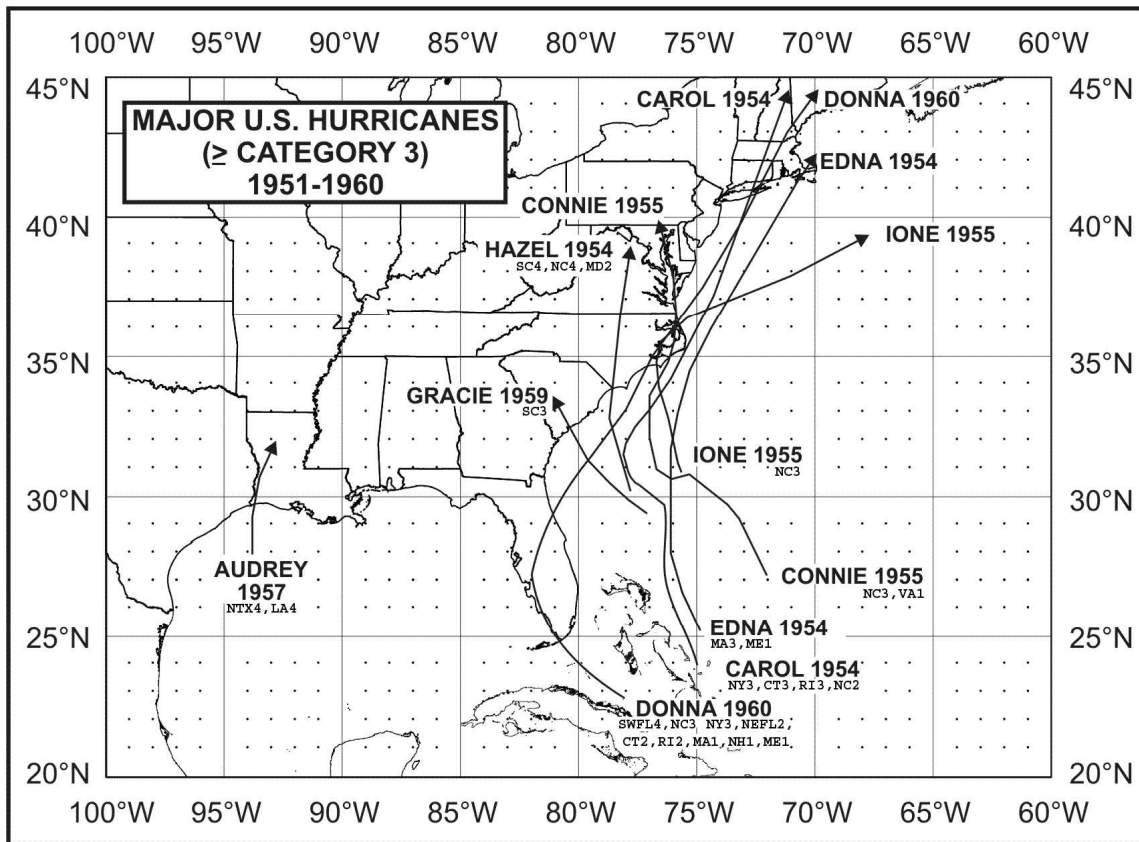
Figure 11. Landfalling United States major hurricanes (stronger than or equal to a category 3) during the period 1951-1960.
