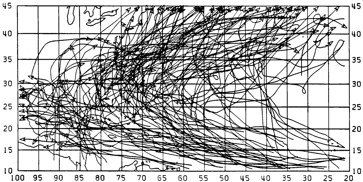
Fig. 5. Tracks of the 141 tropical storms and hurricanes, 1962-1981, used in developing NHC83 model. Portions of storm tracks having initial position \leq 25^\circ\text{N} were used as data set for "South-zone" storms while portions of storm tracks having initial positions > 25^\circ\text{N} comprised the "North-zone" set.
