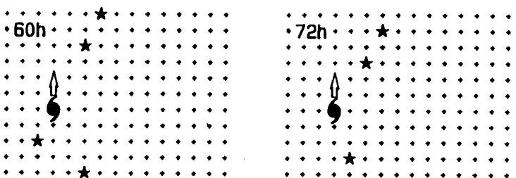
Fig. 13. Predictor location (starred gridpoints) for "perfect-prog" mode (Model 3) over South-zone.
