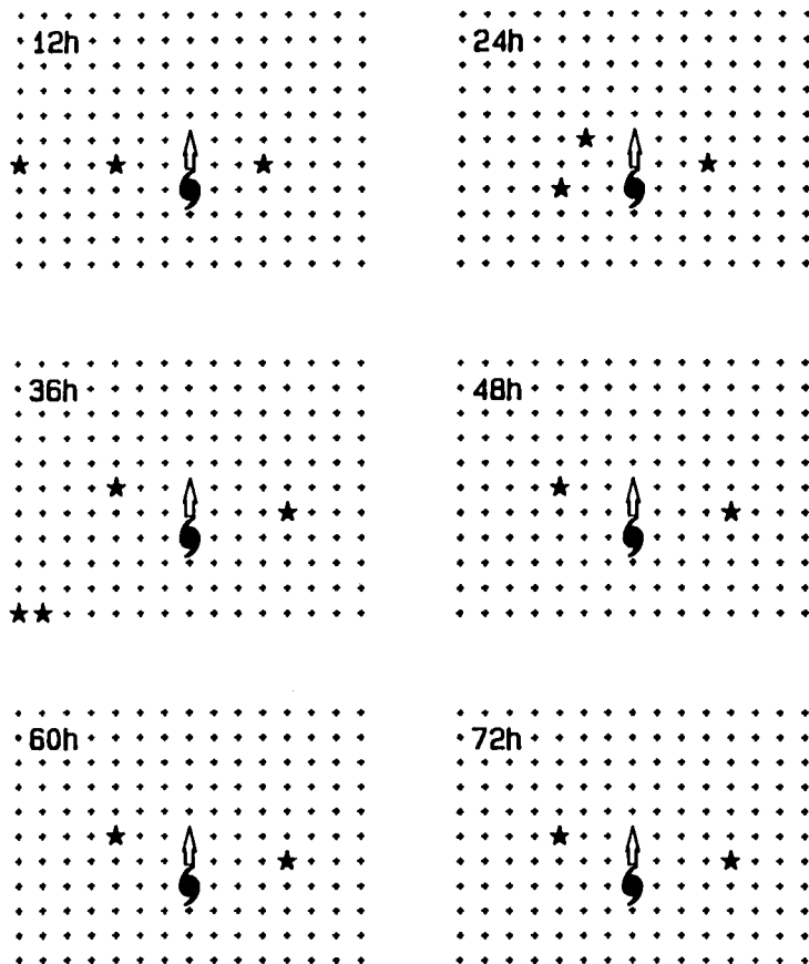
Fig. 12. Similar to Fig. 11 except for North-zone.
