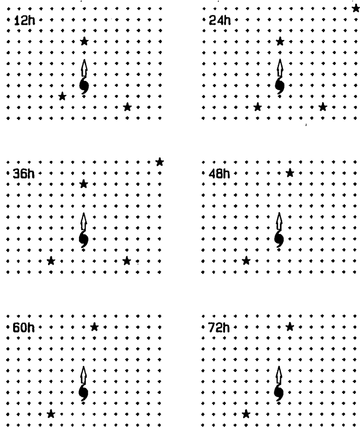
Fig. 12. Similar to Fig. 11 except for North-zone.
