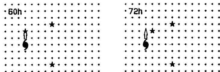
Fig. 11. Predictor location (starred gridpoints) for analysis mode (Model 2) over South-zone.
