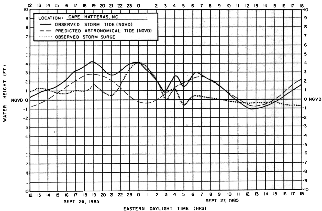
Figure 6. Demonstration of the technique to remove the astronomical tide from the hydrographs shown in Figure 5. Final products are the storm surges generated by Gloria.
