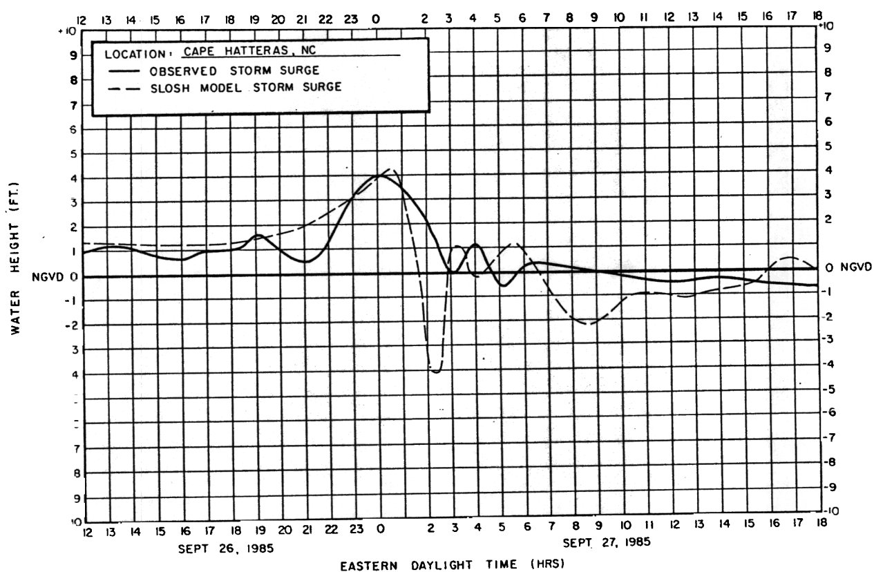
Figure 7a. Comparison of observed versus SLOSH model computed storm surge hydrographs for two locations in Figure 4.
