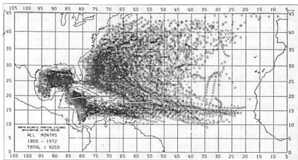
Figure 1. Initial positions of data available for generating a 12-hour prediction equation.
