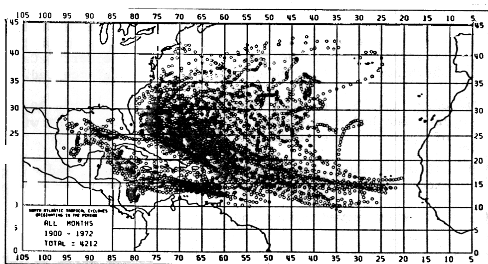
Figure 2. Same as figure 1 except for 72-hours
