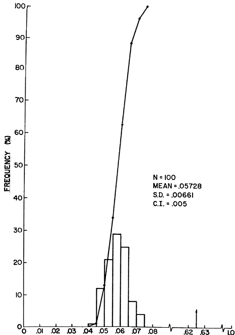
Figure 5. Frequency distribution and cumulative frequency distribution of the multiple correlation coefficients. S.D. = standard deviation. C.I. = class interval
